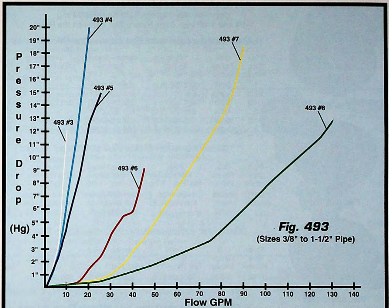
FIG. 493 & 500 - INTAKE WATER STRAINERS DIFFERENTIAL PRESSURE GRAPHS
