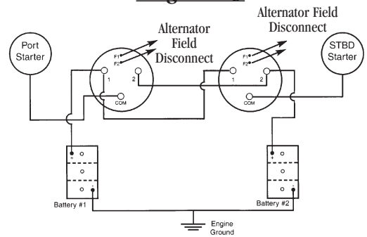
2 SWITCHES, 2 ENGINES, 2 BATTERIES.
