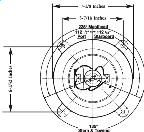
Fig. Nos. 1164 to 1168 Series Double Lens Navigation Light Technical Information (See Lights on Page 45)
