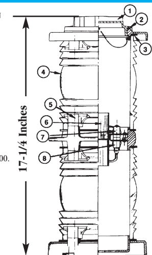
Fig. Nos. 1164 to 1168 Series Double Lens Navigation Light Technical Information (See Lights on Page 45)
