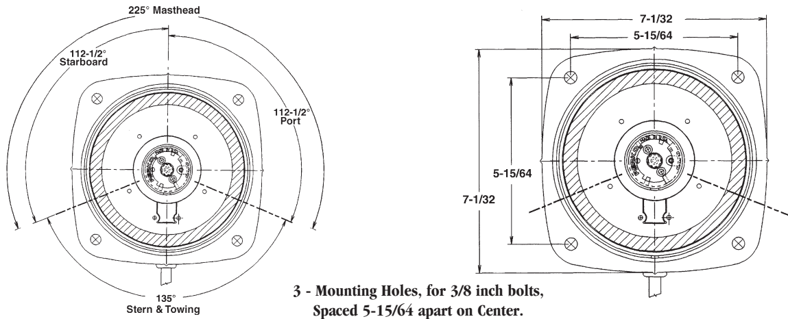
Fig. Nos. 1369 to 1374 Series Single Lens Navigation Light Technical Information (See Lights on Page 42)
