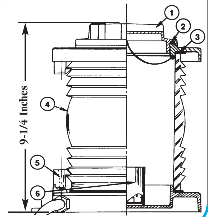
Fig. Nos. 1164 to 1168 Series Double Lens Navigation Light Technical Information (See Lights on Page 45)
