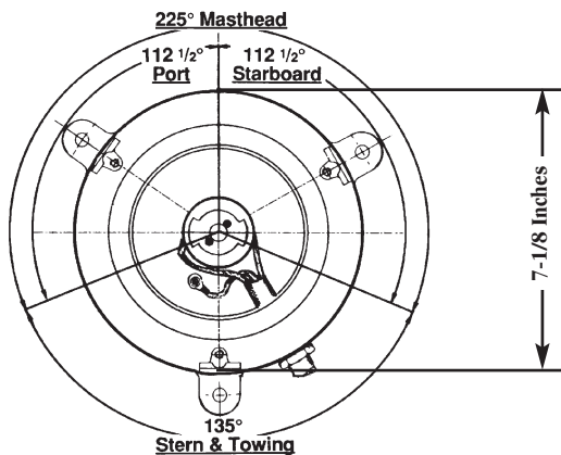
Fig. Nos. 1169 to 1174 Series Single Lens Navigation Light Technical Information (See Lights on Page 44)
