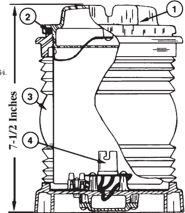
Fig. Nos. 1169 to 1174 Series Single Lens Navigation Light Technical Information (See Lights on Page 44)
