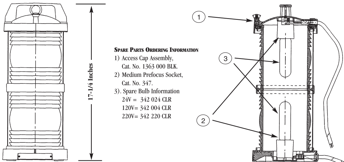
Fig. Nos. 1364 to 1368 Series Double Lens Navigation Light Technical Information (See Lights on Page 43)
