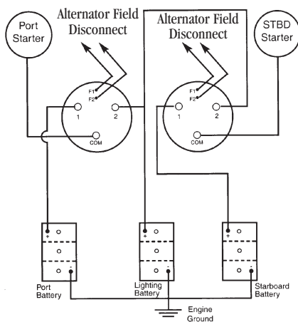
2 SWITCHES, 2 ENGINES, 2 ENGINE BATTERIES AND SEPARATE BANK OF LIGHTING BATTERIES
