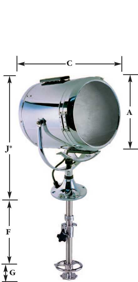
FIG. 885 STANDARD PEDESTAL SHOWN WITH WHEEL CONTROL
