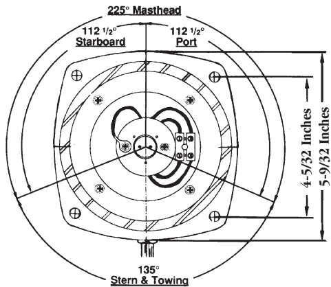
Fig. Nos. 1127 to 1130 Series Navigation Light Technical Information (See Lights on Page 48)
