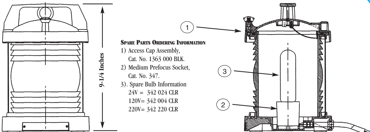
Fig. Nos. 1364 to 1368 Series Double Lens Navigation Light Technical Information (See Lights on Page 43)
