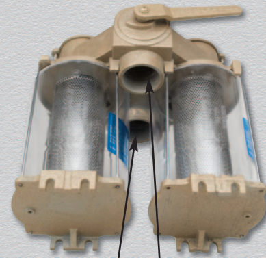
Pipe Connections
