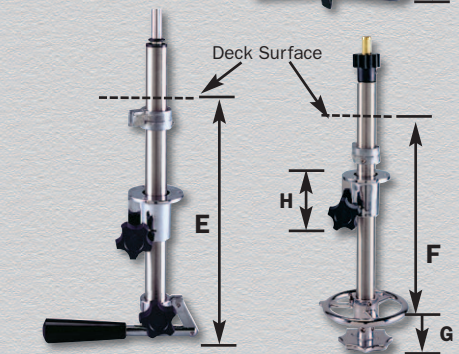
Fig. 0851 Lever Control Fits 0305 Head
